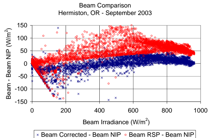
Fig. 9: Beam Comparison for September, 2003 at Hermiston, OR. Symbols are the same as in Fig. 7.
