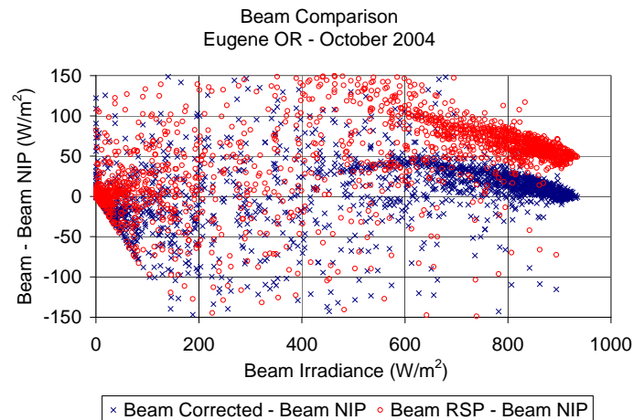
Fig. 8: Beam comparison for October, 2004. Symbols are the same as in Fig. 7.
