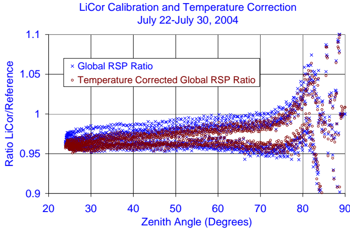
Fig. 1: Calibration of a LiCor pyranometer. The reference global value is the sum of diffuse obtained by a Schenk Star pyranometer and an Eppley NIP pyr heliometer projected onto the horizontal surface. x's show the ratio of the LiCor to the reference global values. Circles show the same comparison with a solar cell temperature correction applied.
